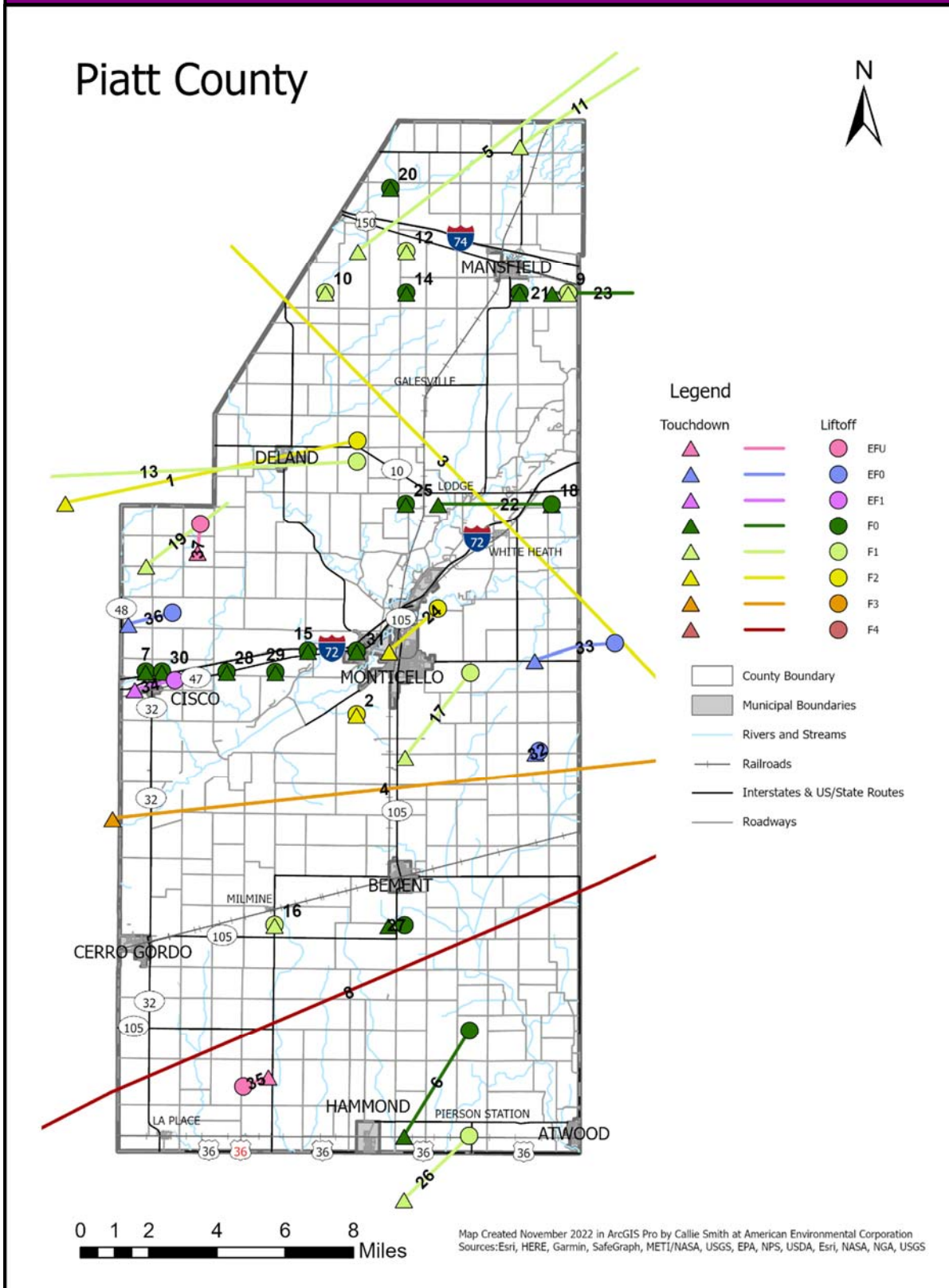
Figure T-4 Tornado Pathways in Piatt County
